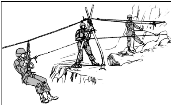
Figure 10-27. SUSPENSION TRAVERSE
