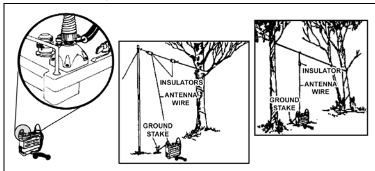
Figure 7-4. MODIFIED CONNECTION AT TOP OF ANTENNA
