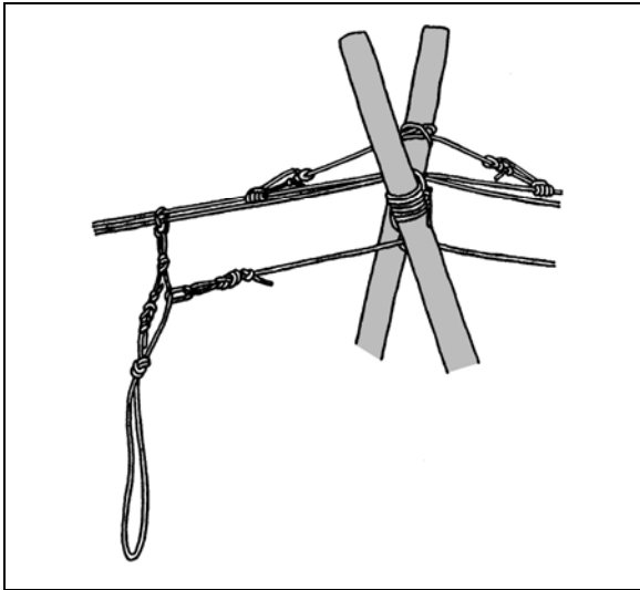
Figure 10-27. SUSPENSION TRAVERSE
