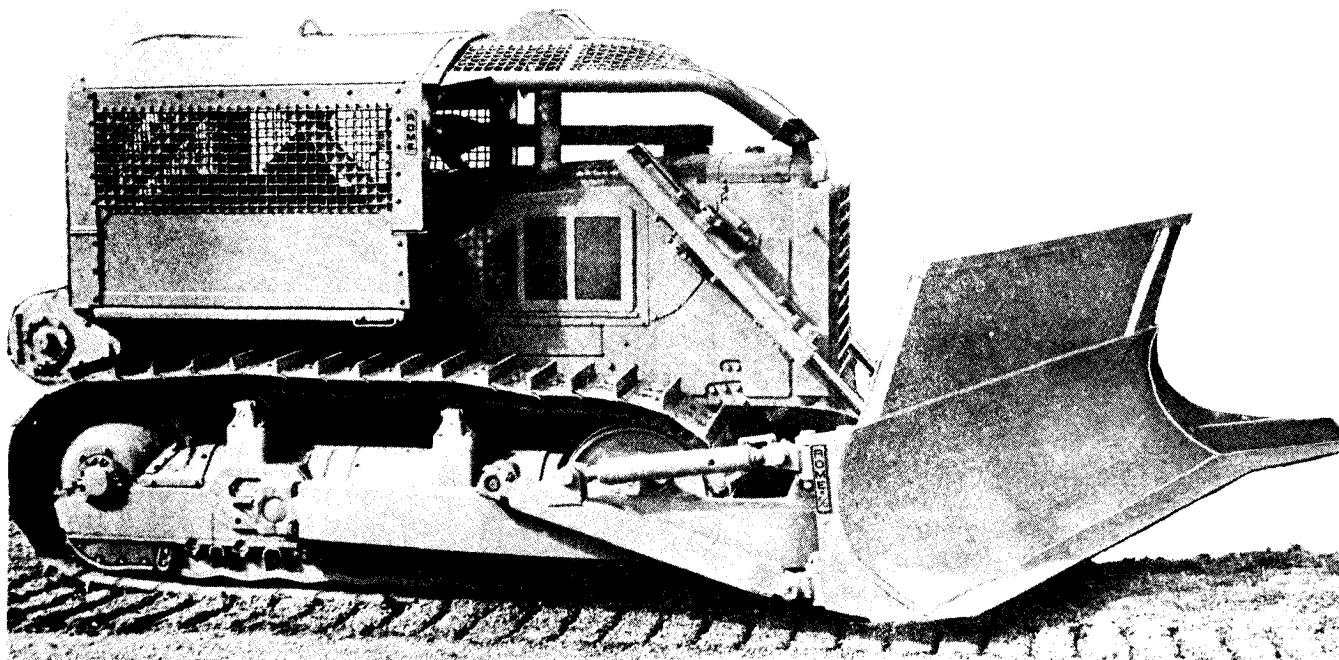
Figure B-4. D9G clearing tractor equipped with perforated engine side panels, hydraulic lift cylinder protection, louvered radiator grill guard, remote air intake, extra heavy duty jungle clearing cab, and Rome K/G shearing blade.
