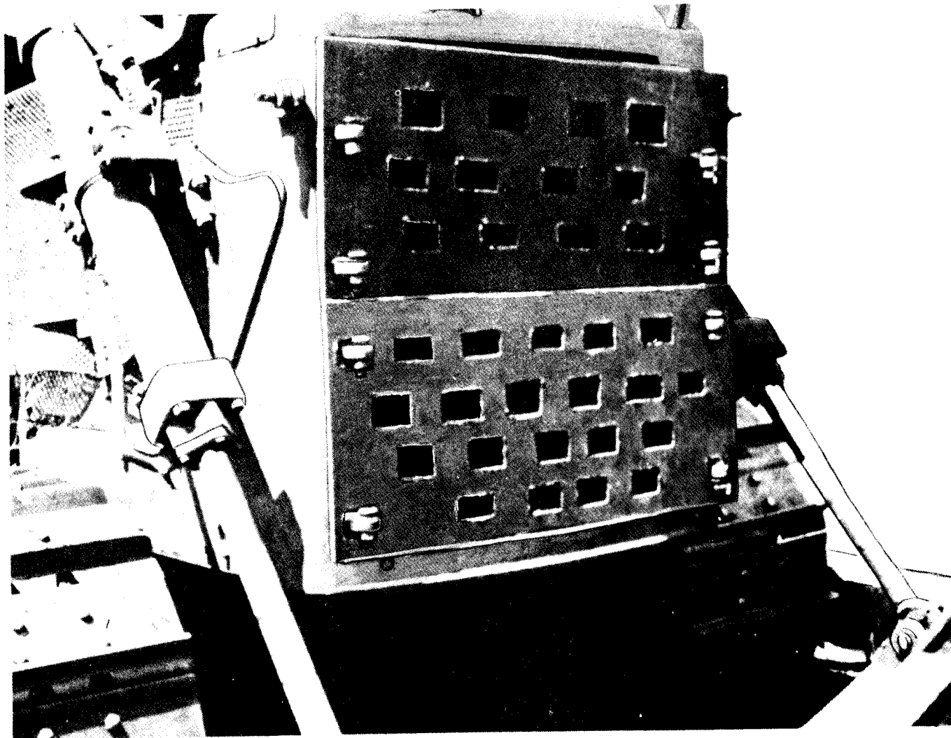
Figure B-2. A cutout steel plate used for expedient radiator protection. This device severely restricts airflow through the radiator.
