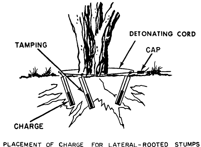
Figure 3-31. Stump blasting charges.
